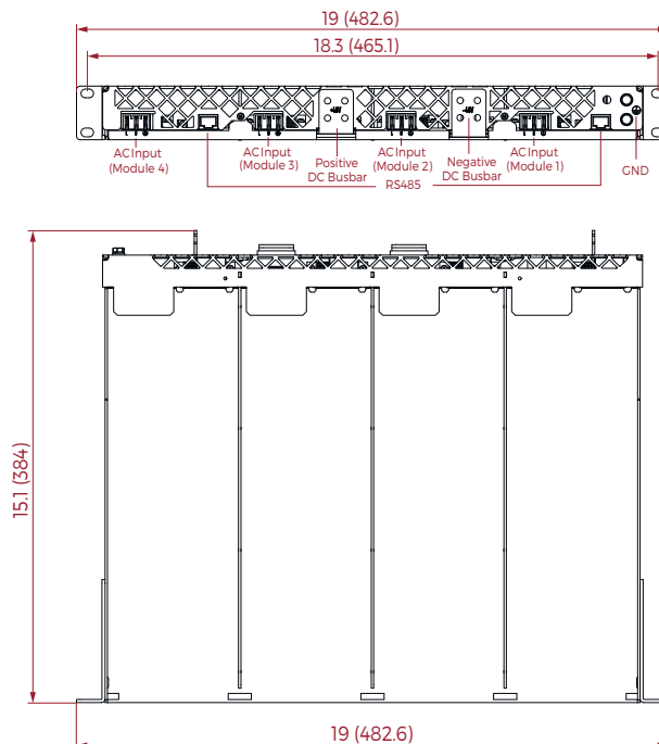
XG1948G - Top and rear view with position and description of connectors
